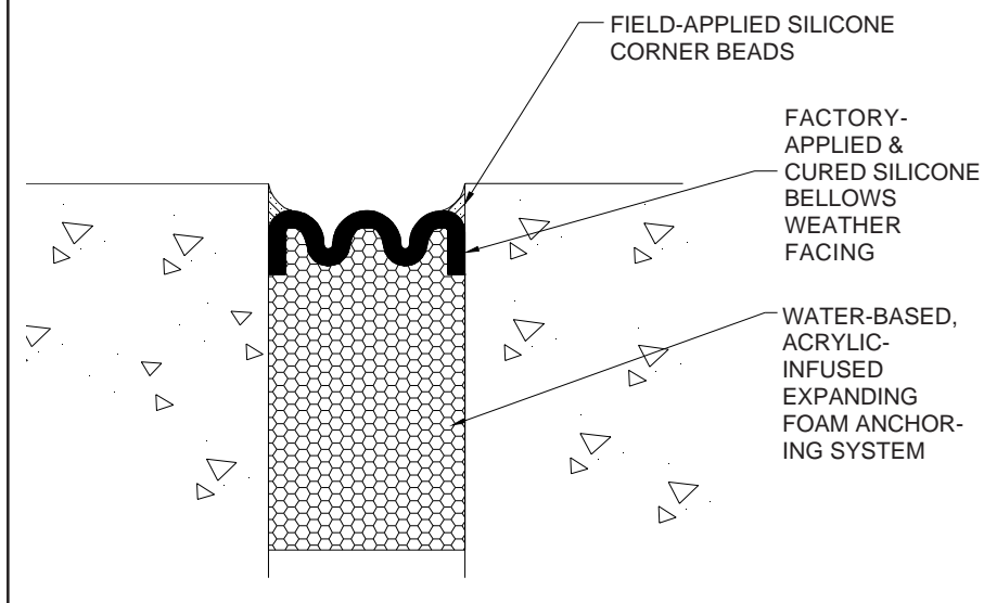
Figure 1: SEISMIC COLORSEAL in Typical Installation (Substrates may vary.)
