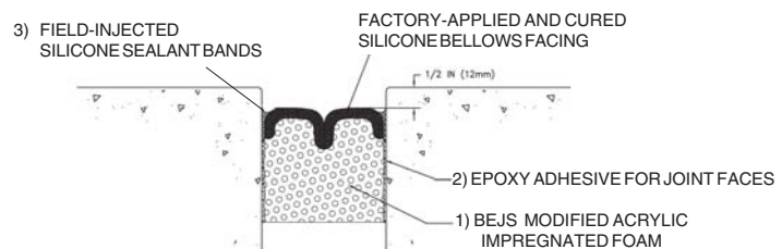
Fig. 2: BEJS SYSTEM in Existing Steel Angles--Retrofit
