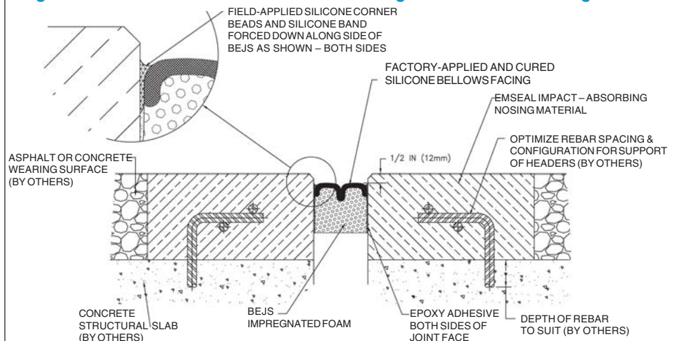
Fig. 3: BEJS SYSTEM in New or Rebuilt Joint Edges with EMSEAL Nosing Material
